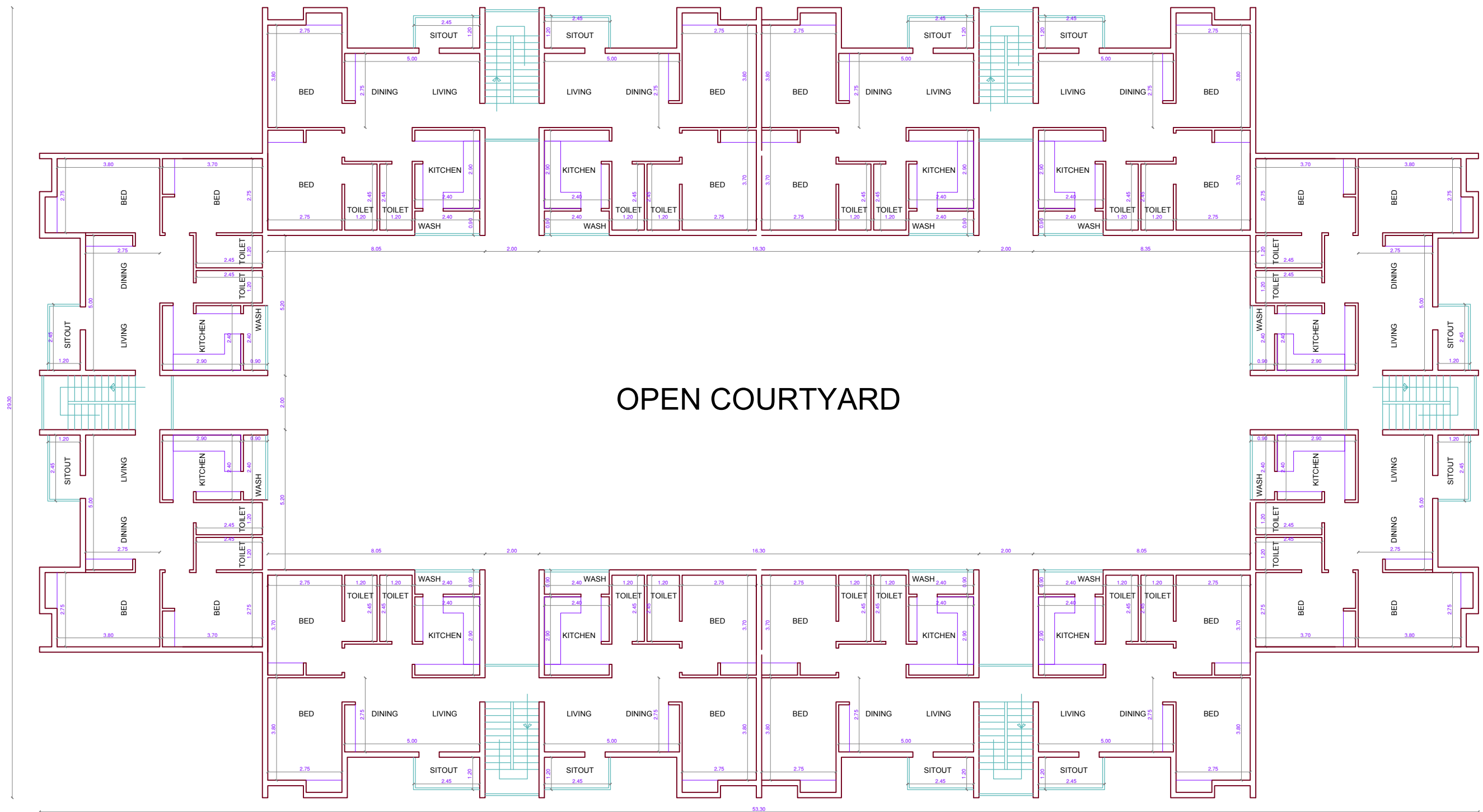
TYPICAL FLOOR PLAN ( 1 to 3 FLOORS )
